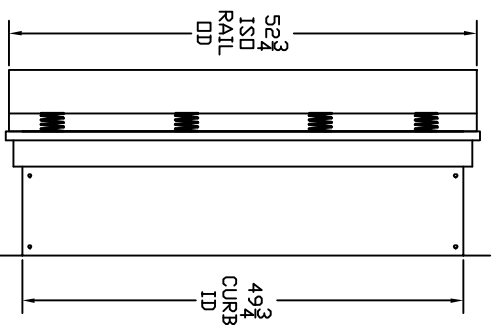
RIGHT VIEW
