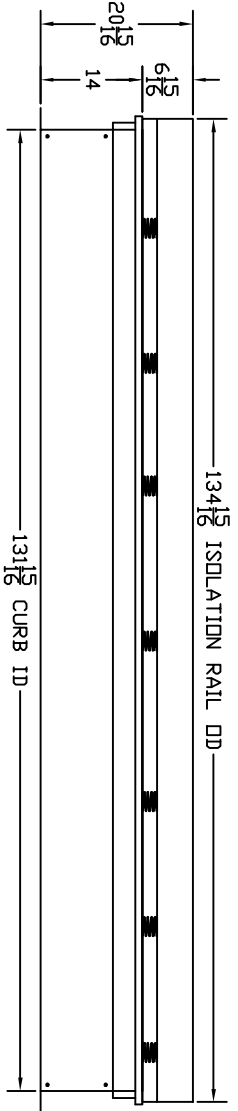
FRONT VIEW
