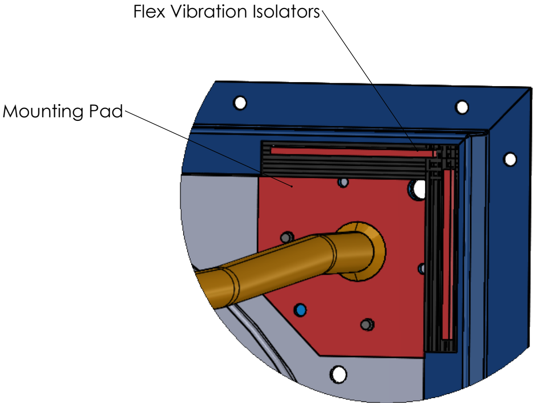
DETAIL A SCALE 1 : 2
